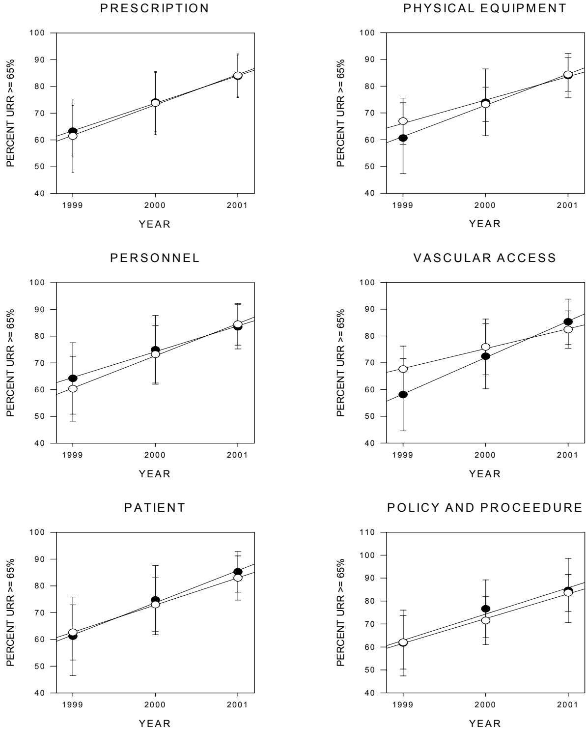
Figure 2. Plots of the mean of the percentage of patients in a facility with a URR \geq 65\% in the intervention facilities that targeted a factor (o) and did not target a factor (•). The targeted factor is listed above the individual plot.
